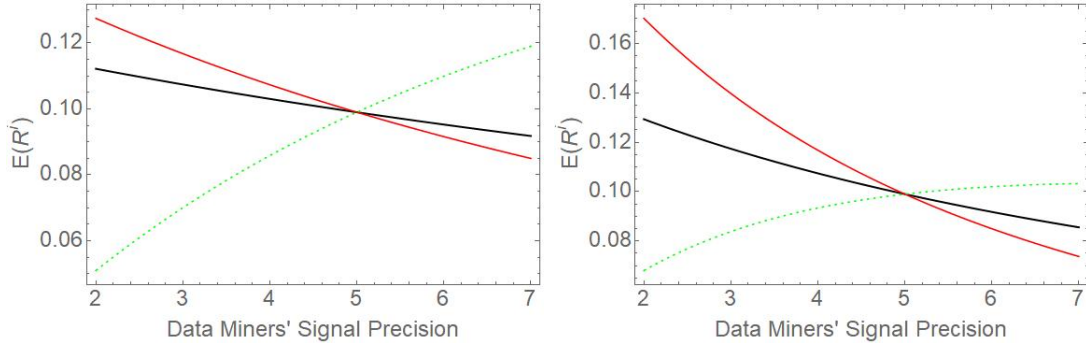
Figure IA.1: Left Panel: \mu = 0.1 . Other parameter values: \sigma_v^2 = \sigma_\eta^2 = 1 , \rho = 0.5 , \tau_{ex} = 5 . Right Panel: \mu = 0.4 . Other parameter values are as in the left panel. In each case the figure shows the effect of a variation in the precision of data miners' signals ( \tau_{dm} ) on (i) experts' gross expected return, \bar{R}(\tau_{ex}) (red line), (ii) data miners' gross expected return, \bar{R}(\tau_{dm}) (green dashed line) and (iii) asset managers' average gross return, \bar{R}^A (plain black line).
